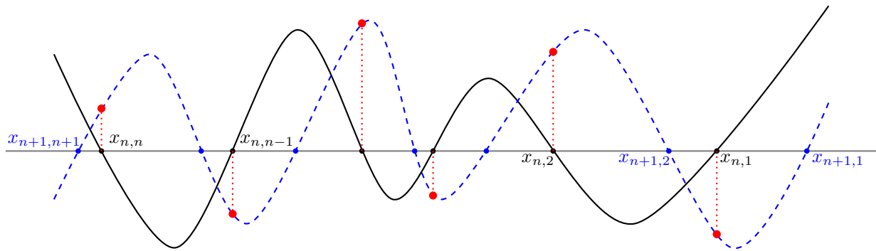
Figure 2.1: The interlacing zeros of P_n(x) and P_{n+1}(x) .
